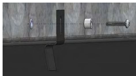
Figure 52 - Z-Bracket for .625" panels
