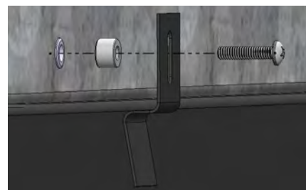
Figure 51 - Z-Bracket for .375" panels
