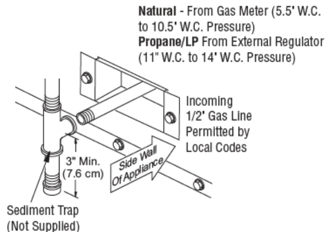
Figure 26 - Sediment Trap
