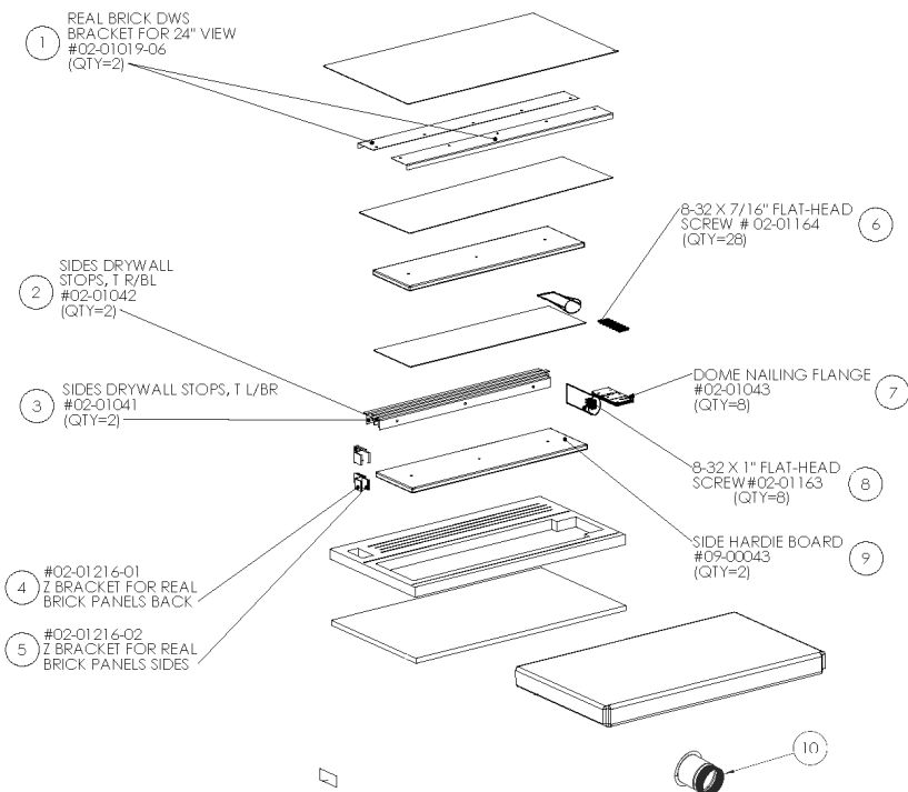
Figure 56 - Accessory Kit
