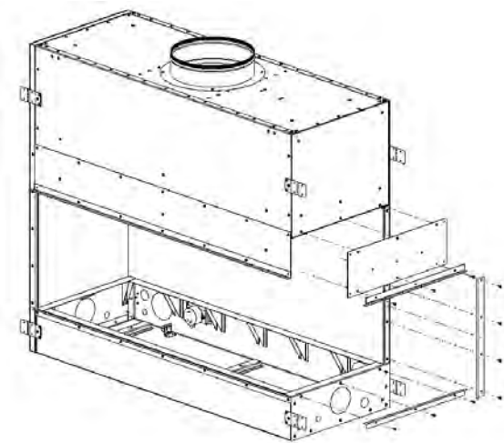
Figure 54 - Right Reduction Kit
